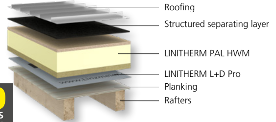
LINITHERM PAL HWM for metal roofs with visible rafters
