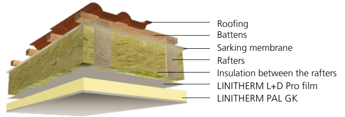
LINITHERM PAL GK in new construction with full rafter insulation
