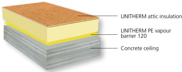
Insulation on concrete attic floor that can be walked on and loaded
