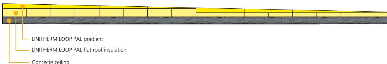
Layering principle: LINITHERM gradient insulation plus flat roof insulation
