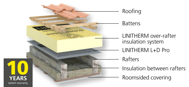
Over-rafter insulation system with existing insulation between rafters
