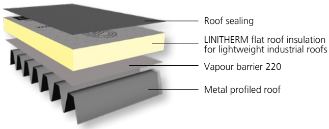
LINITHERM PAL FD for metal roofs
