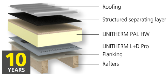
LINITHERM PAL HW for metal roofs with visible rafters
