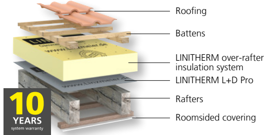
Over-rafter insulation system with roomsided covering
