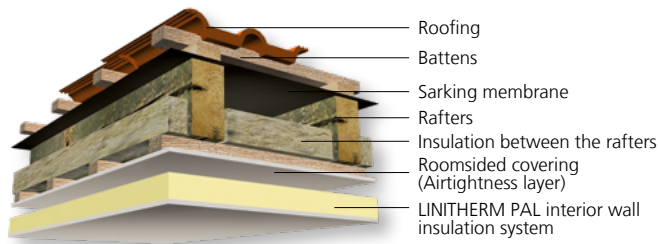
LINITHERM PAL GK with existing insulation between the rafters
